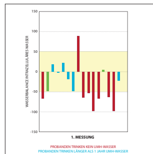
BIACORPUS-MEASUREMENT WITHOUT UMH (EXCEPT BLUE)
